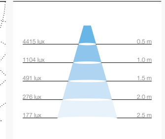
Illuminance Chart
